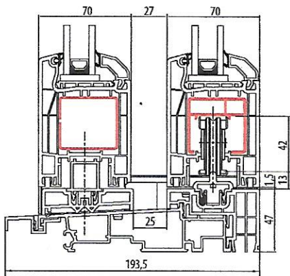
ALUPLAST HST 70
