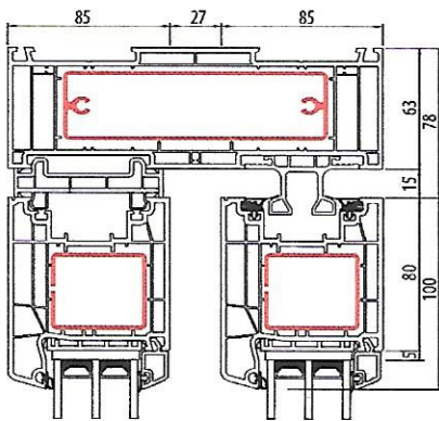
ALUPLAST HST 70
