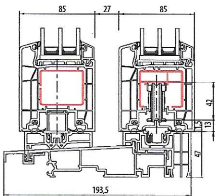
ALUPLAST HST 85
